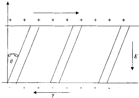
Fig.1 Schematic of ER structure at the initial stage
