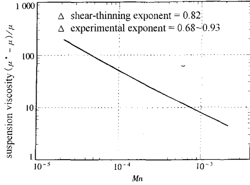
Fig.6 The non-dimensional suspension viscosity (\mu^* - \mu)/\mu versus Mason number in the log-log plot
