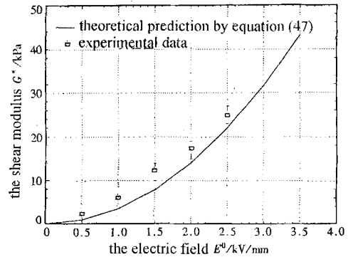
Fig.2 The shear modulus versus the applied electric field
