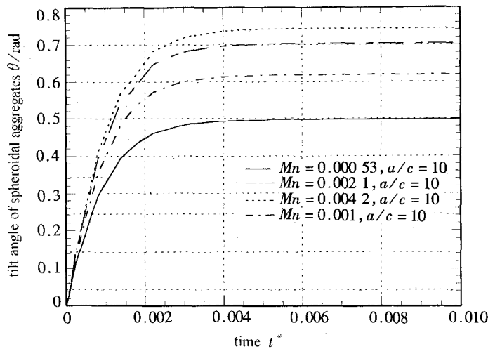
Fig. 4 The rotational angle as a function of non-dimensional time t^* = t\gamma_{13} for different Mason number Mn
