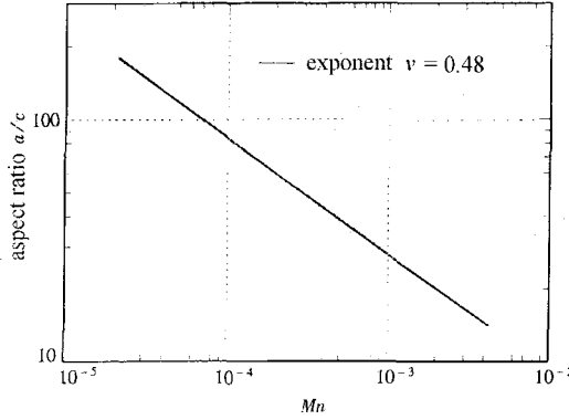
Fig.5 The aspect ratio a/c versus Mason number in the log-log plot
